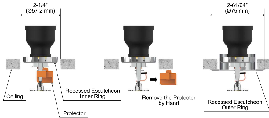
Figure 6: Protector Removal
